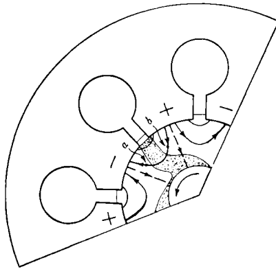
FIG. 1-25.—Diagram showing focusing action of r-f fields on space charge.
